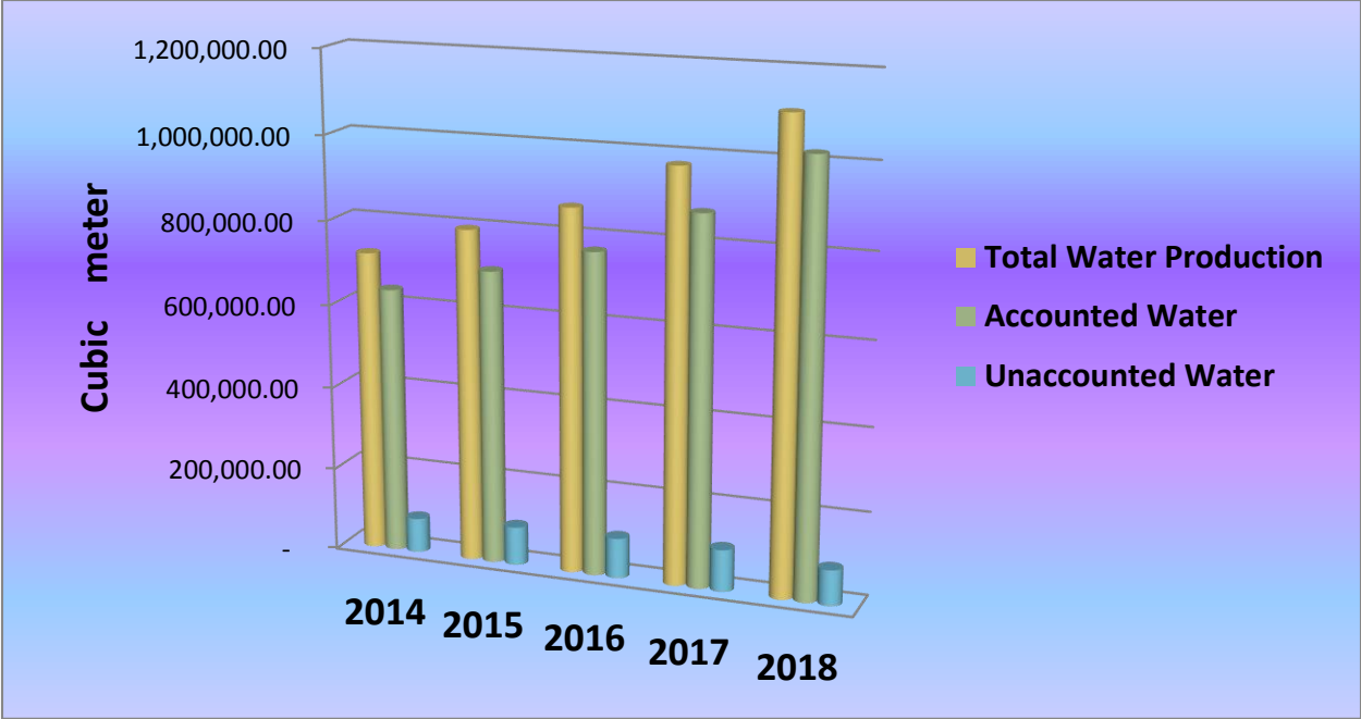
Water Production Flow Chart
